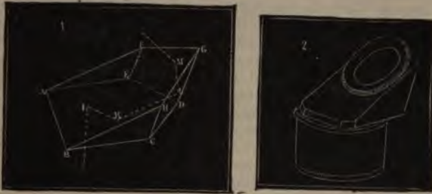
Nacet's Erecting-Prism.
